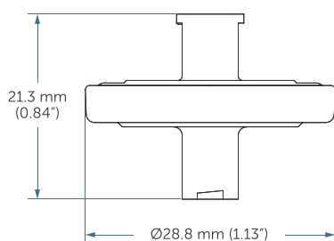
ProcessGard Lab Disk Disposable 25 Size Black shell type
