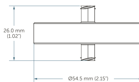
ProcessGard Lab Disk Disposable 50 Size Black shell type
